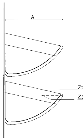
Starco Jumbo 8 elevator buckets in a welded version (parameters in mm)
