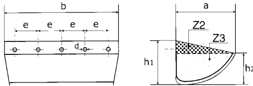
Starco elevator buckets in a welded version (parameters in mm)
